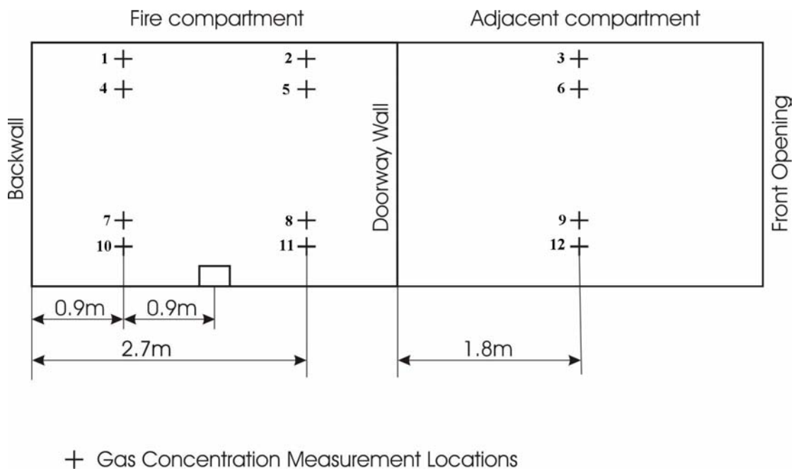
Figure 2.13. A side elevation of the gas concentration measurement probe locations for probes 1-12.
